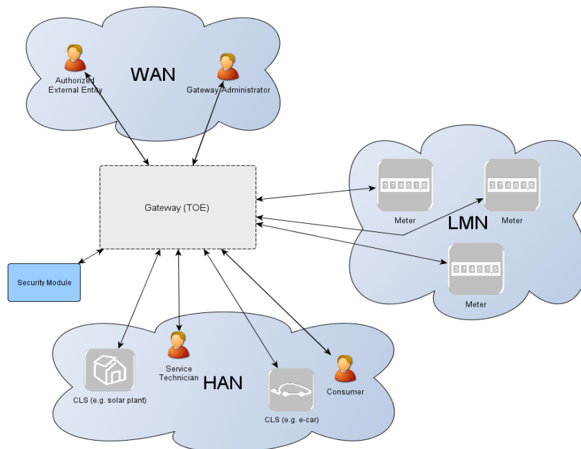
Figure 1: The TOE and its direct environment
