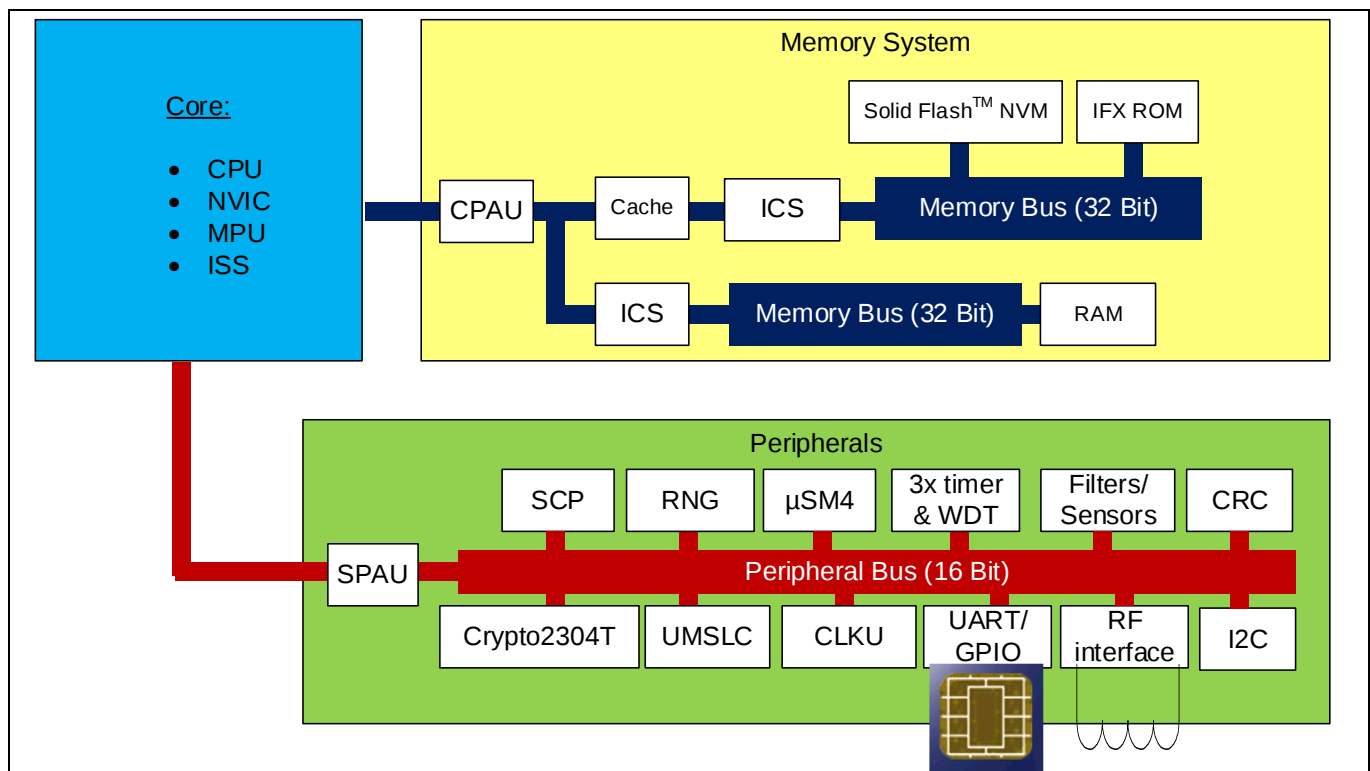
Figure 1 Block diagram of TOE hardware
