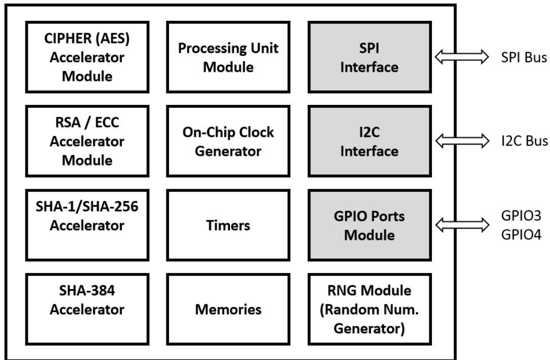
Figure 1 – TPM2.0 Block Diagram
